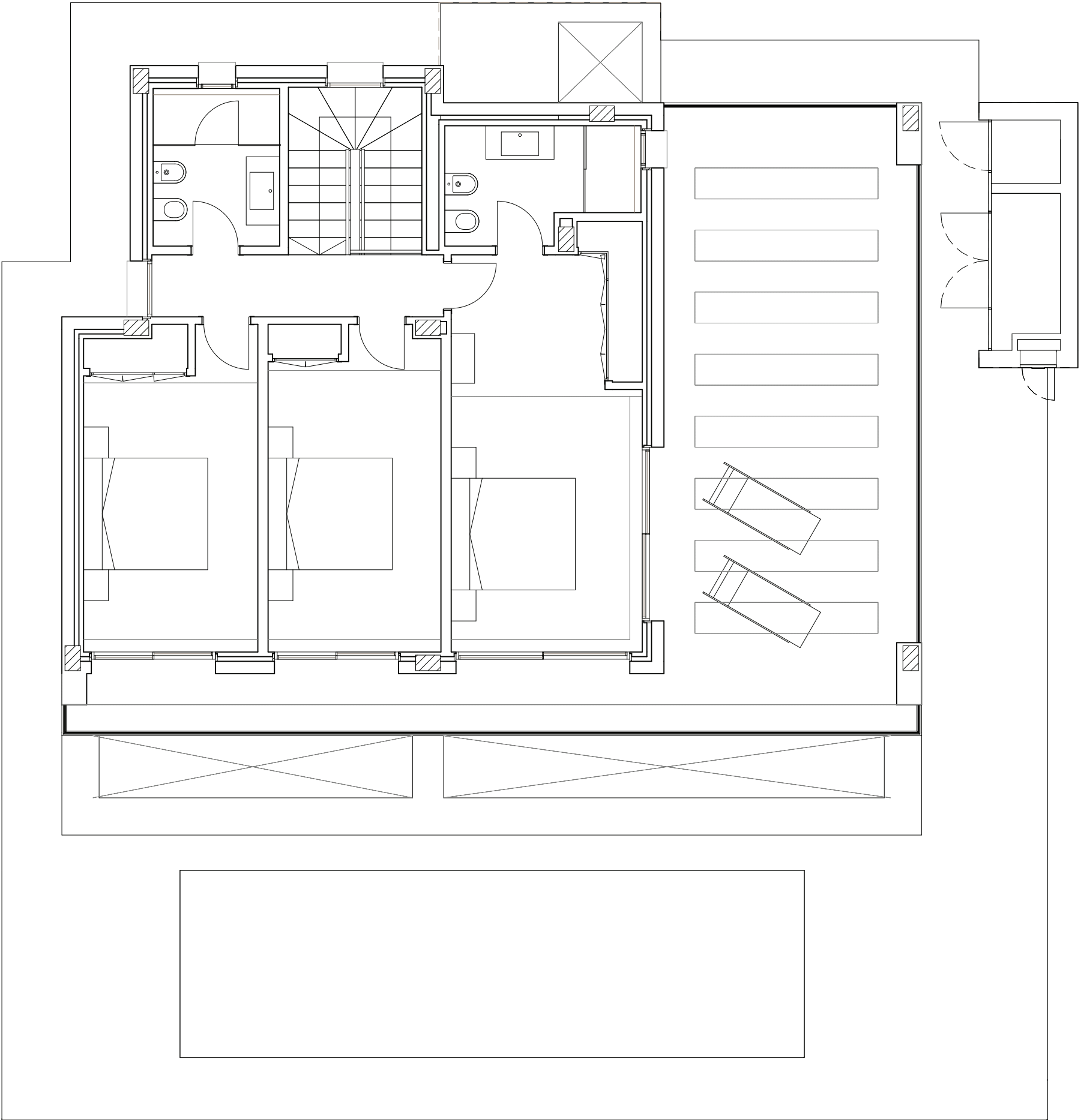
FIRST FLOOR
