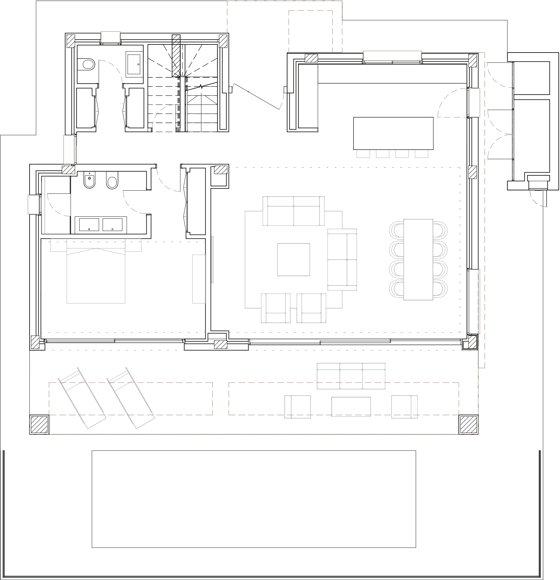
GROUND FLOOR
