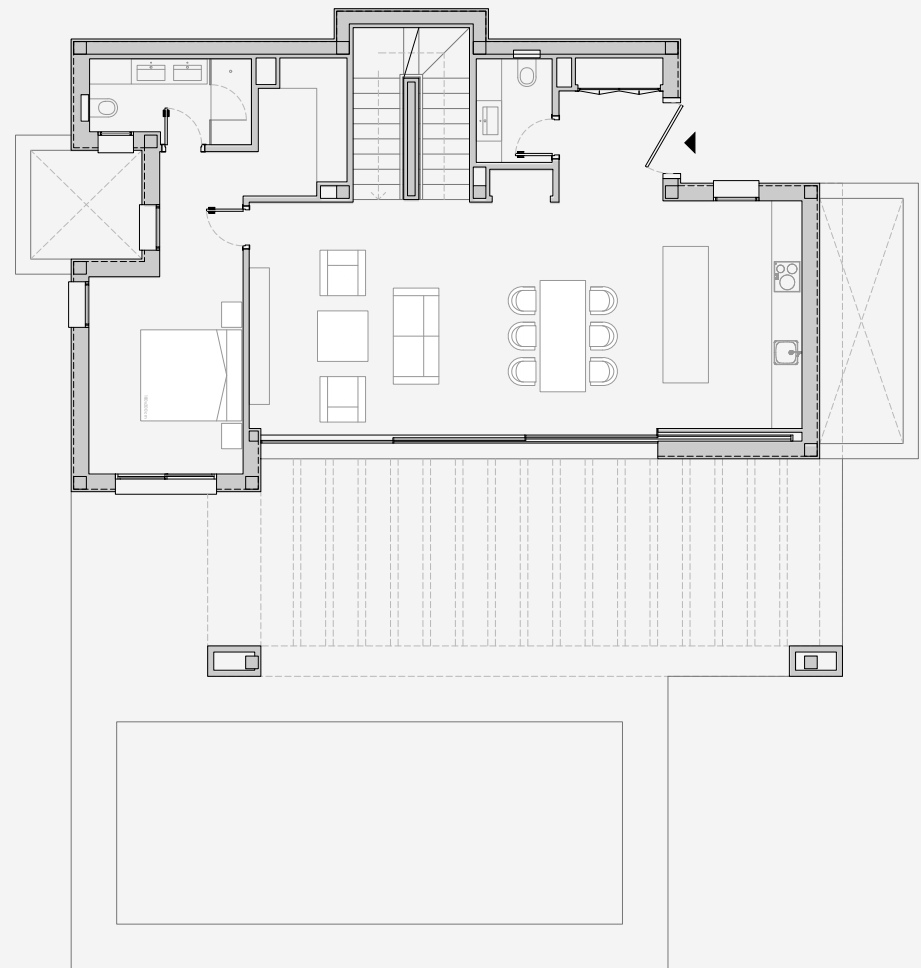
VILLA OLIVO GROUND FLOOR
