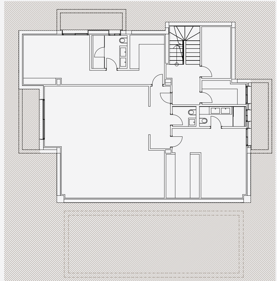
VILLA LAUREL S-B BASEMENT
